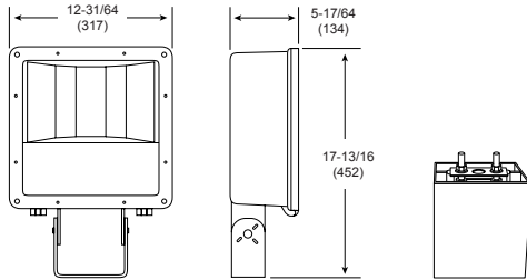
[ PM ] 6" Long Pole mount Arm
